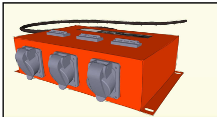
Floor/Wall mount Splitter Box with 1x Input & 3x panel mount Outputs on trailing leads with circuit protection & integrated 3-Phase Remote Power/KWh Meter.
