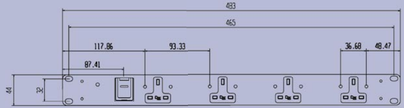
T-04H 4 WAY 1U HORIZONTAL
