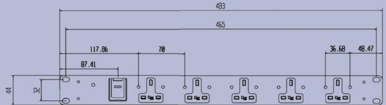
T-05H 5 WAY 1U HORIZONTAL
