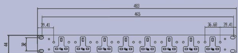
T-08H 8 WAY 1U HORIZONTAL
